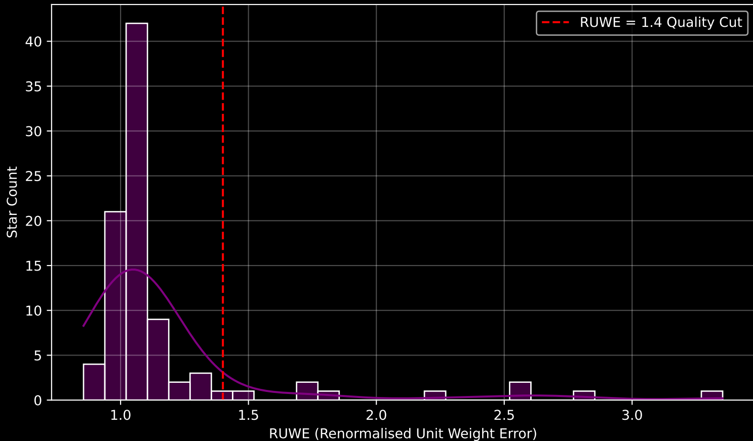
GAPOGEE DR17 Field [K2_C2_354+18] RUWE Distribution (n= 91)
