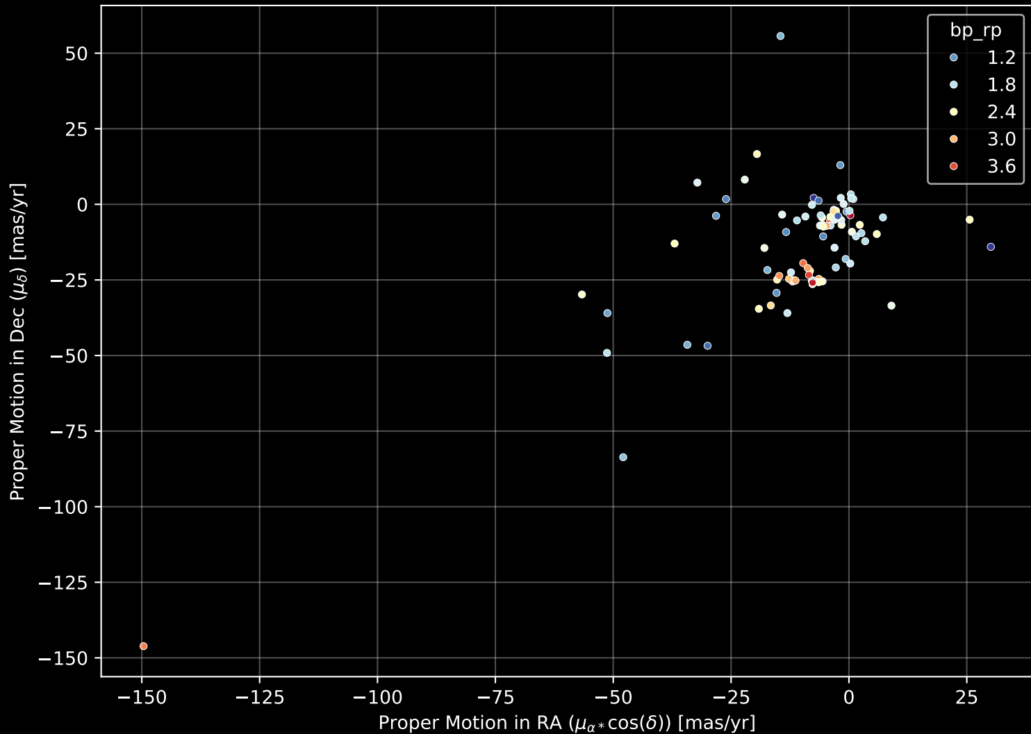
APOGEE DR17 Field: [K2_C2_354+18] Proper Motion Diagram (n= 93)
